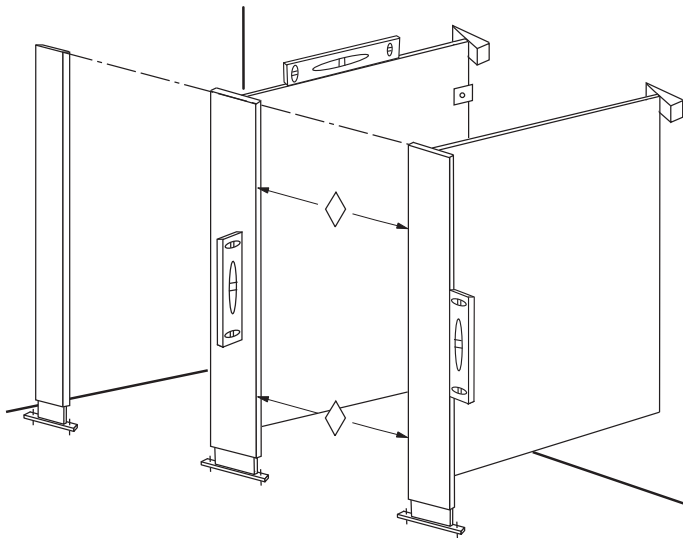
Fig. 6b: Floor-Anchored Installation.
