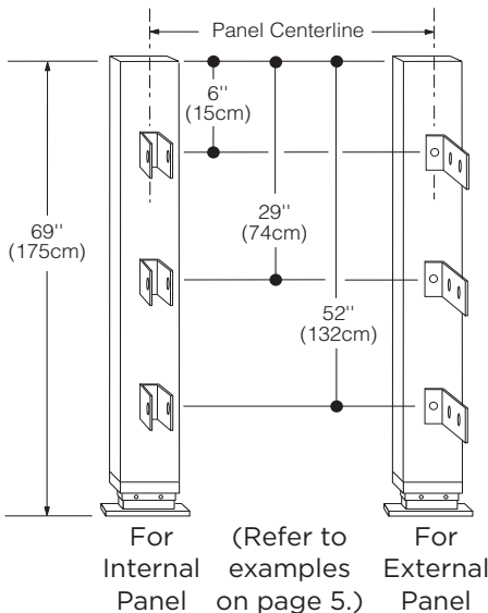
Fig. 5a: Floor-Anchored or Ceiling-Hung Bracket Placement.
