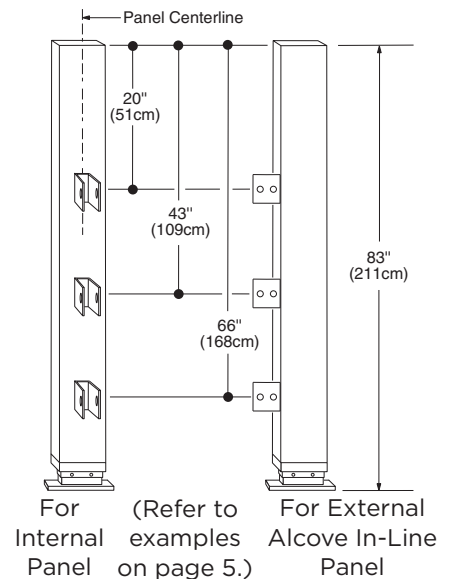
Fig. 5c: Floor-to-Ceiling Anchored.
