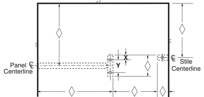
Fig. 1c: Floor-Anchored or Ceiling-Hung Alcove Closed Layout. Inswing Door
