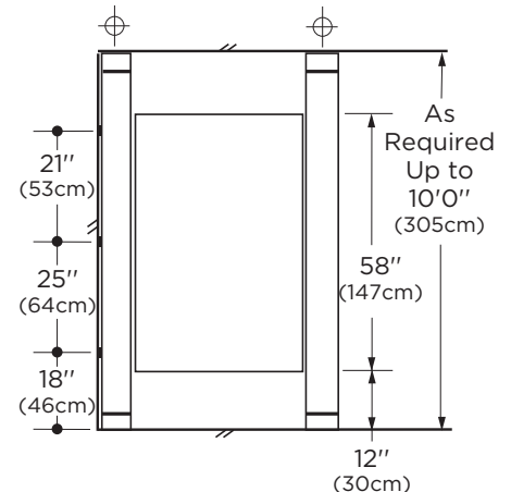
Fig. 5c: Floor-to-Ceiling Anchored.
