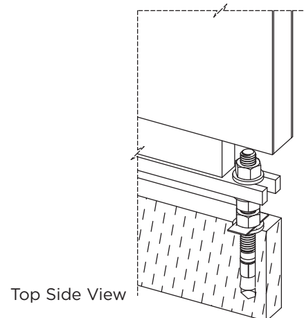
Fig. 2b: Floor Anchor Attached to Stile. (3-Dimensional View)
