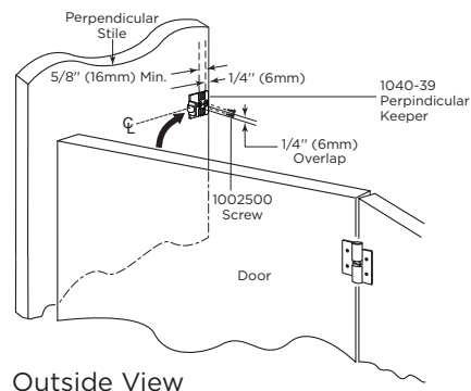
Fig. 9b: Outwing Door Keeper on Perpendicular Stile (Alcove Layout).
