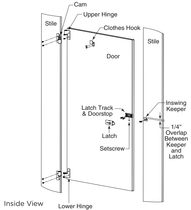
Fig. 8a: Right-Hand Inswing Door.
