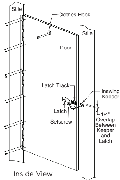
Fig. 8a: Right-Hand Inswing Door.
