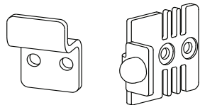
#1040-35 Inswing Keeper #1040-39 Perpendicular Keeper
