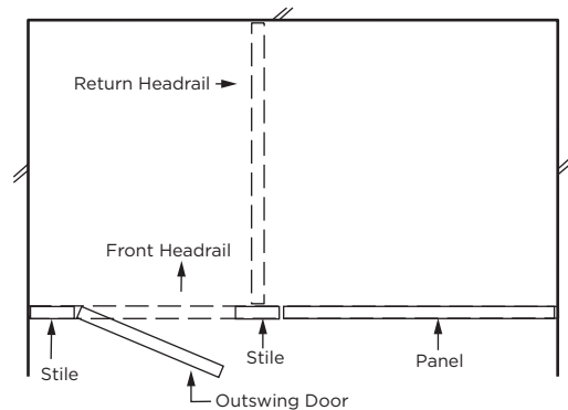
Fig. 7c: Alcove Configuration.
