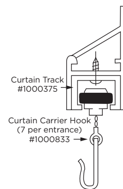
Fig. 7b: Curtain Track
