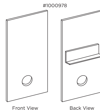
Fig. 7d: Detail of End Cap
