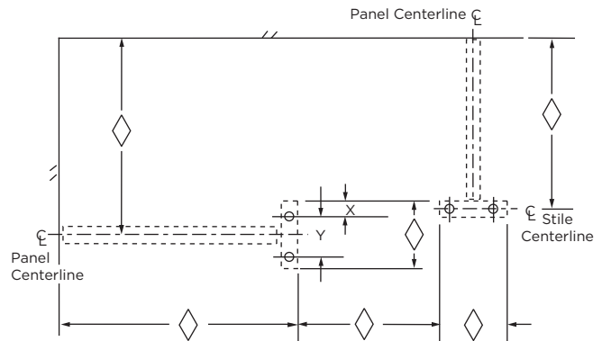
Fig. 1b: Floor-Anchored or Ceiling-Hung Alcove Open Layout.
