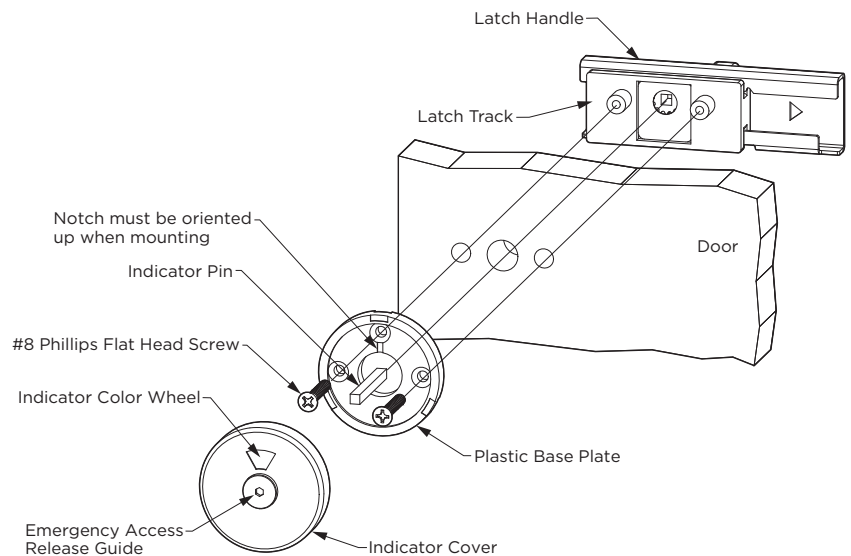
Fig. 9b: Occupancy Indicator Latch Packet
