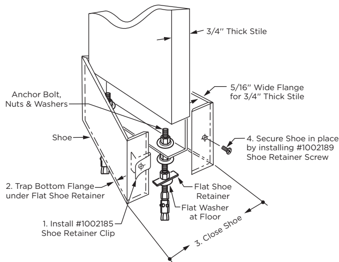
Fig. 14a: Standard Stile Installation.
