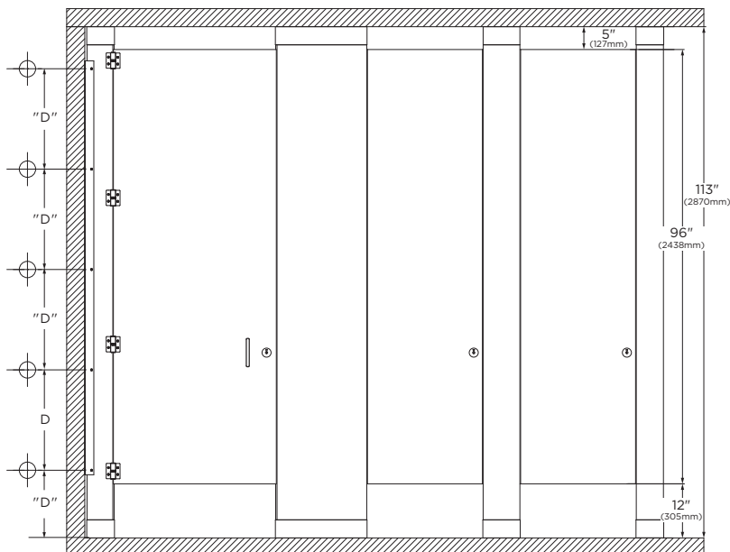
12" (305mm) AFF Partition Elevation
