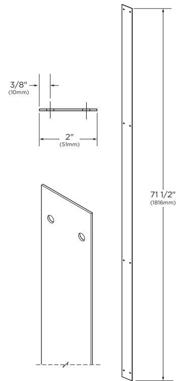
#1002389 Strip Bracket
